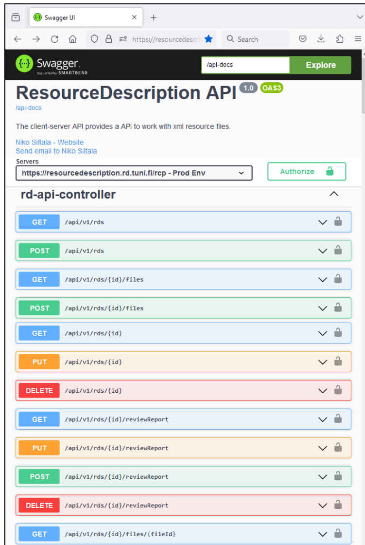
Figure 6: A few endpoints of RCP backend application represented in Swagger UI
