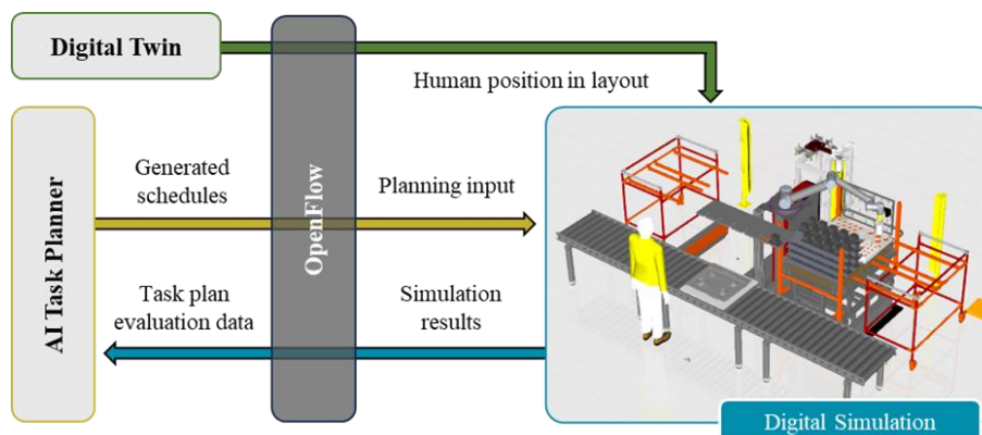
Figure 66: ODIN AI task planner module integration with OpenFlow, Digital Twin and Digital Simulation modules
