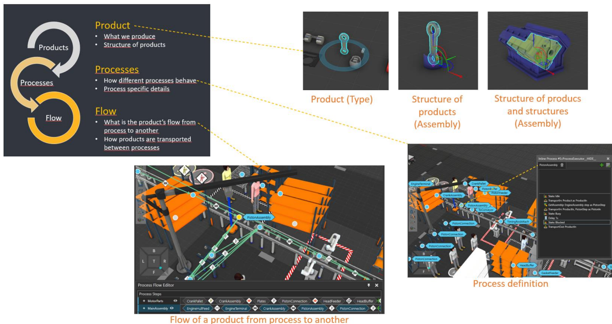
Figure 46: Details of the simplified motor assembly using PM in a HRC cell
