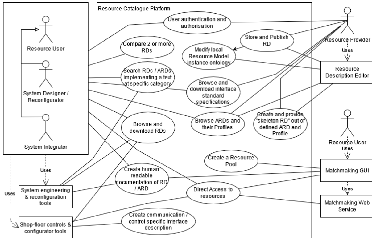
Figure 4: Use cases for Resource Catalogue Platform [6]
