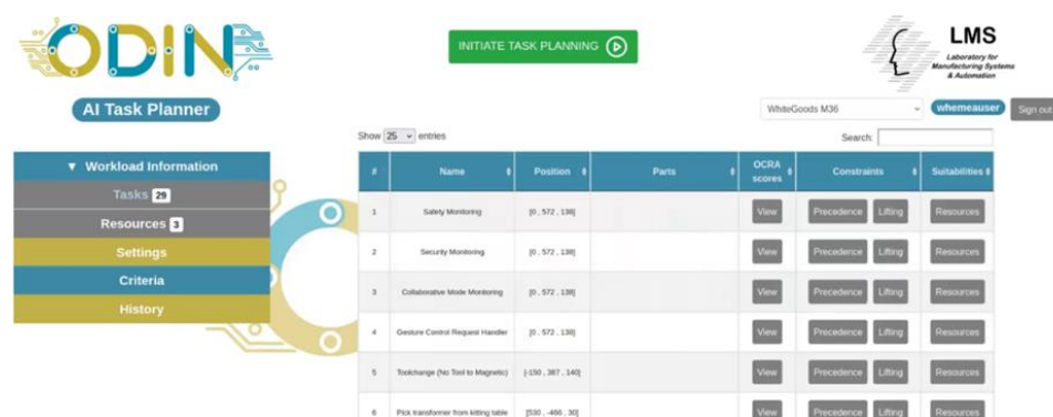
Figure 71: AI Task Planner UI – Workload information tab
