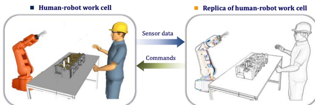
Figure 32: The general representation of the digital twin for HRC cells
