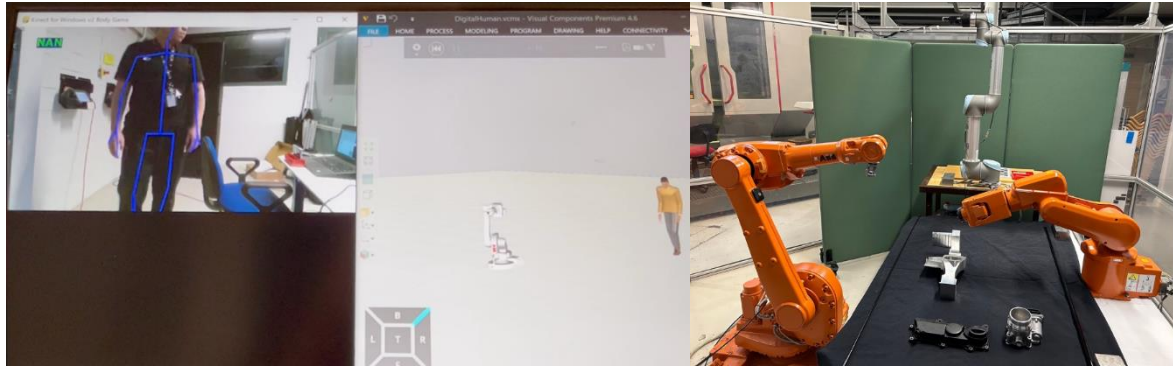
Figure 40: An overview of the physical HRC system and its digital twin system in KTH pilot case
