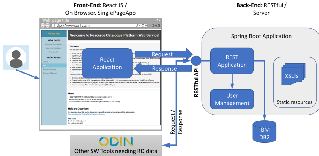
Figure 5: Architecture of Resource Catalogue Platform
