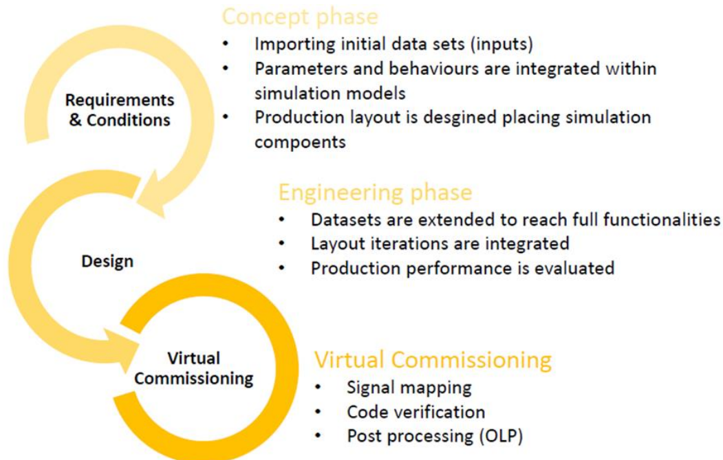
Figure 44: Detail of the phases concept, design, and virtual commissioning phases implemented in ODIN
