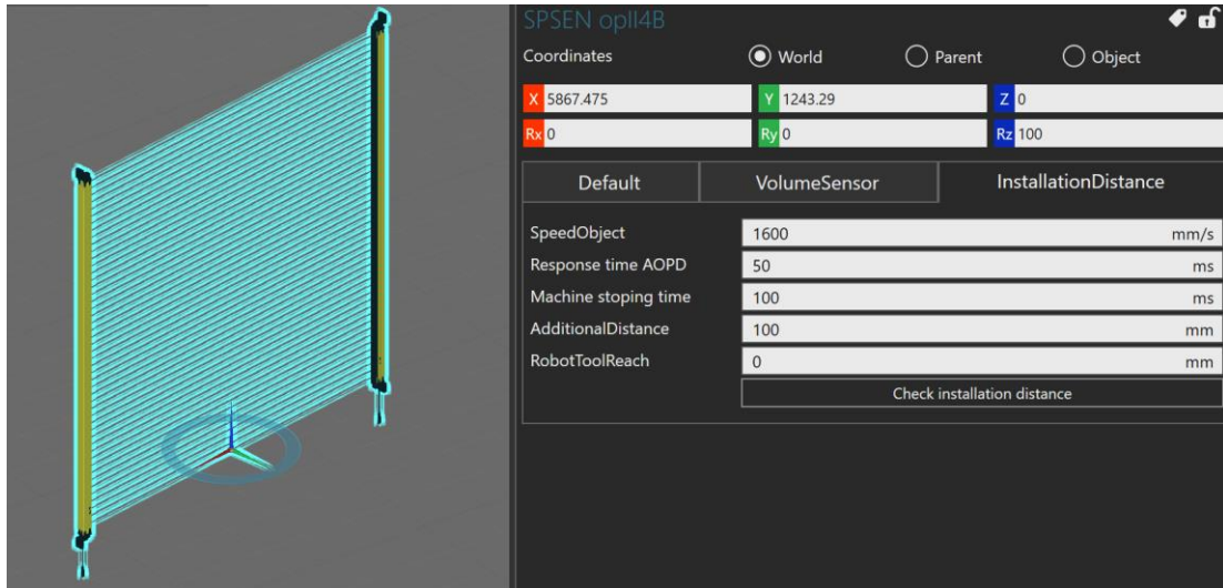
Figure 58: Safety Distance component and UI with access to the functionalities
