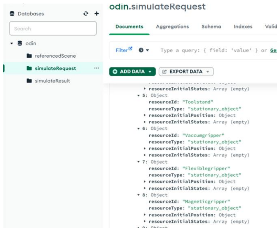
Figure 64: MongoDB database for Simulated layout initialization
