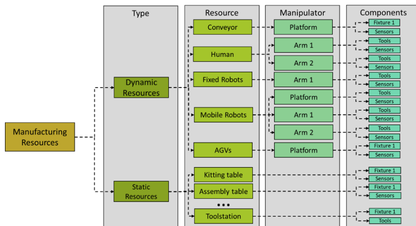
Figure 63: ODIN Resources hierarchical model
