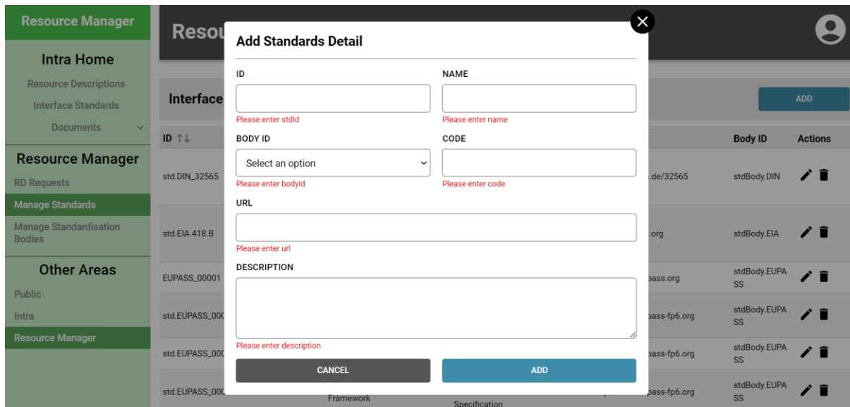
Figure 27: Notification of Error Message for Incomplete Information
