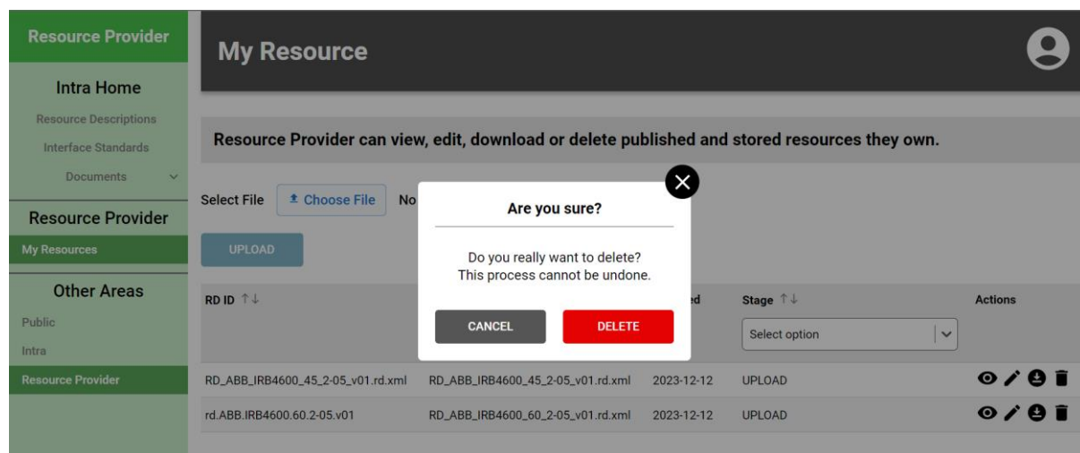
Figure 18: User Interface of warning message when deleting RD
