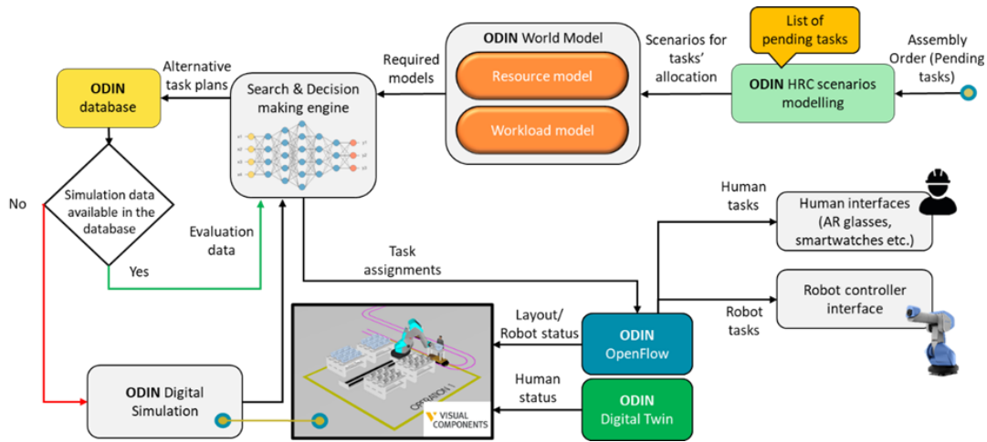
Figure 65: ODIN AI task planner module methodology
