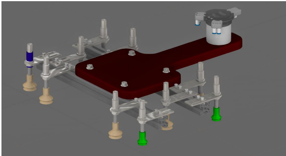
Figure 49: Vacuum Gripper for Whirlpool pilot
