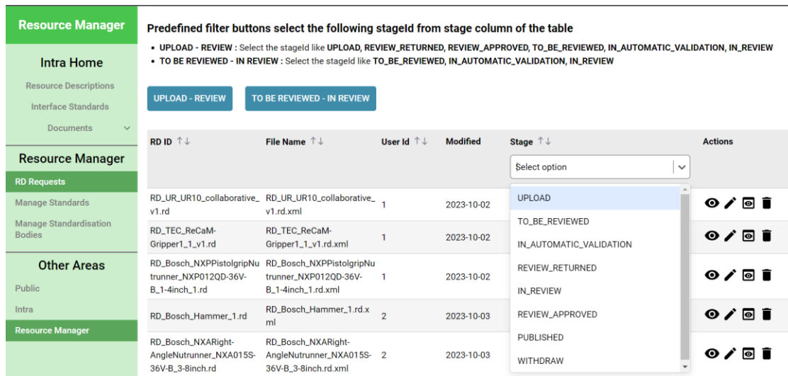
Figure 22: User Interface of Filtering RD by Resource Manager
