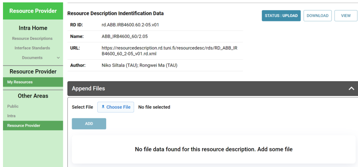
Figure 17: User Interface of Attaching RD's connected data
