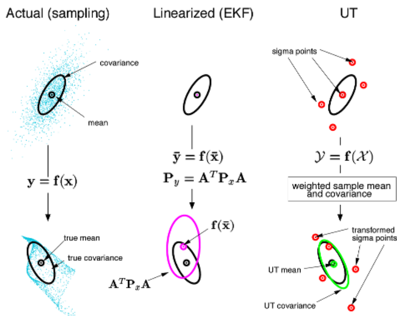
Figure 35: An overview of Unscented Kalman Filter (UKF)
